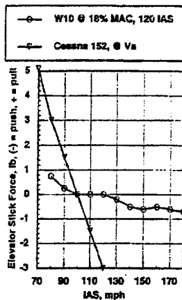
Figure 1. Static Longitudinal Stability (Stick force gradient)
