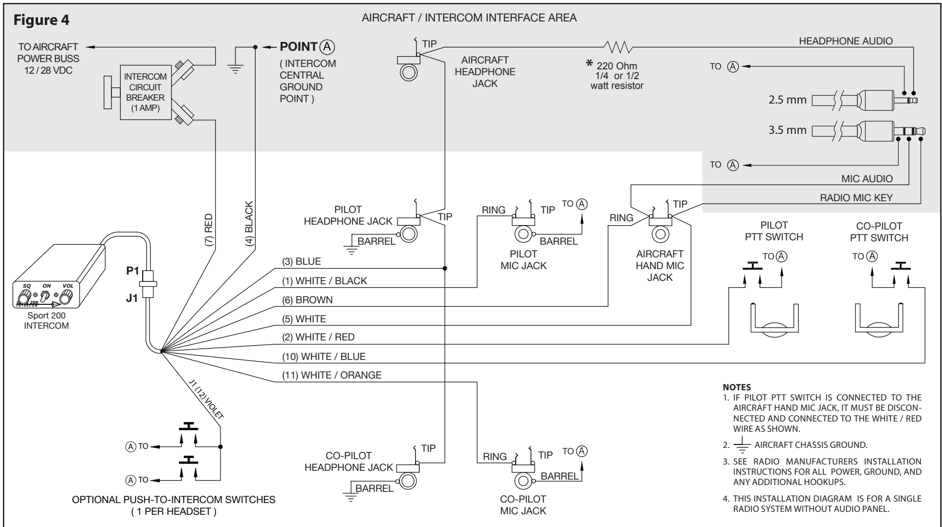
Sport 200 – Sporty’s SP-200 Radio Installation Wiring Diagram
